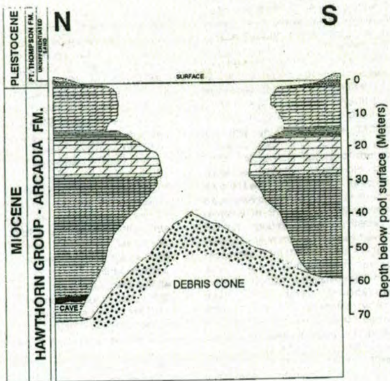
Figure 2. A cross section of Warm Mineral Springs. Source: Sarasota County/Jennifer Steadman Ryan
