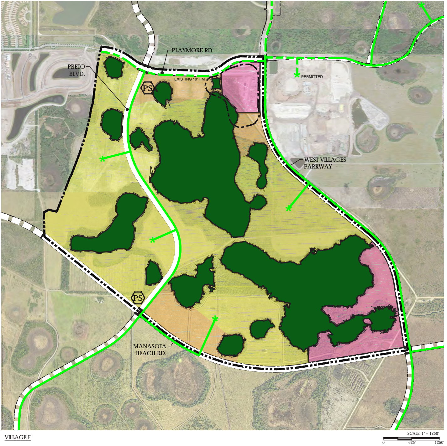
Figure 3.5.1.B. Wastewater Systems Plan
