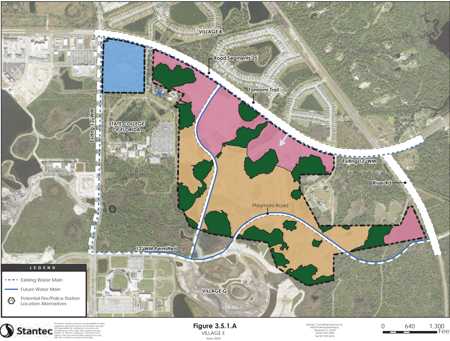
Figure 3.5.1.A Water System Plan
